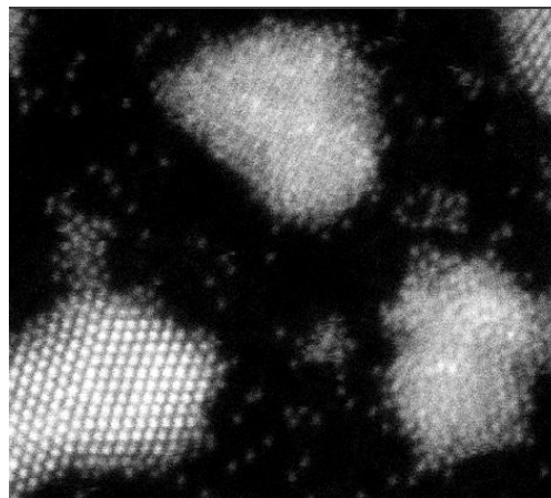
STEM image of platinum atoms on electrodes of fuel cell
