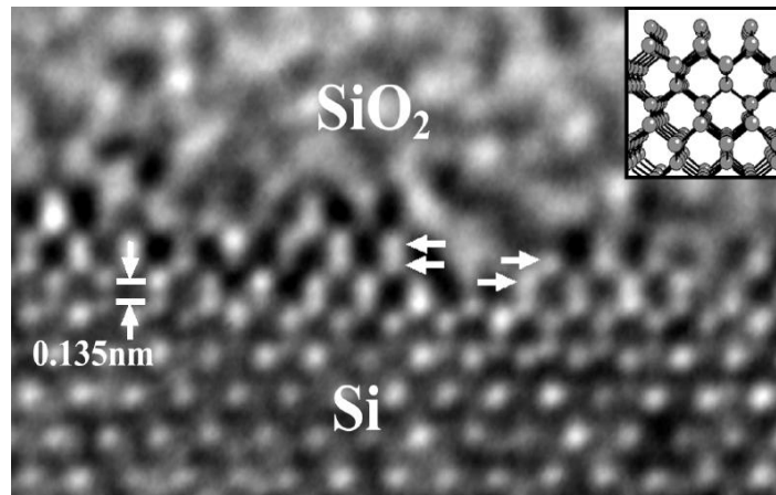
High-resolution TEM image of an interface between silicon and silicon oxide
